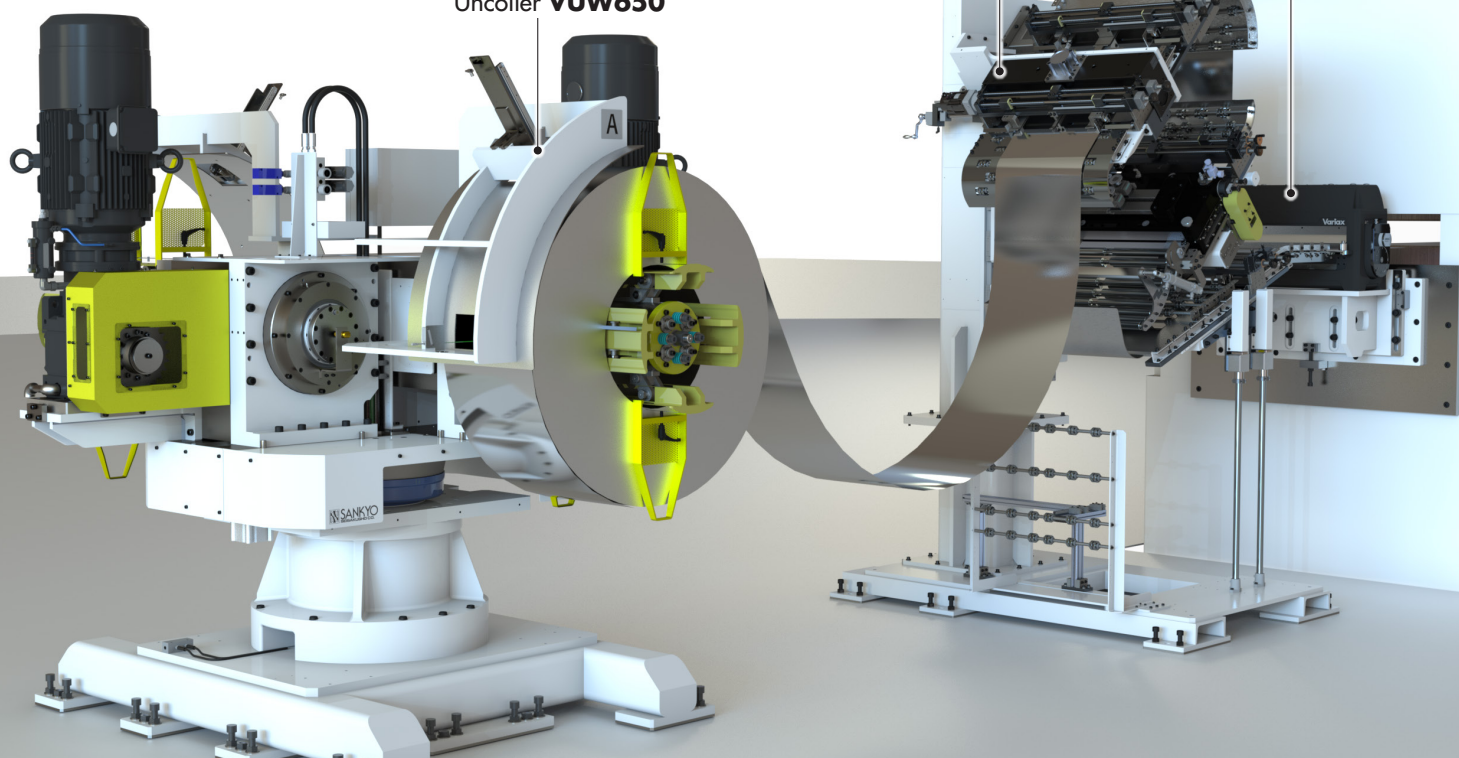
Uncoiler VUW650
